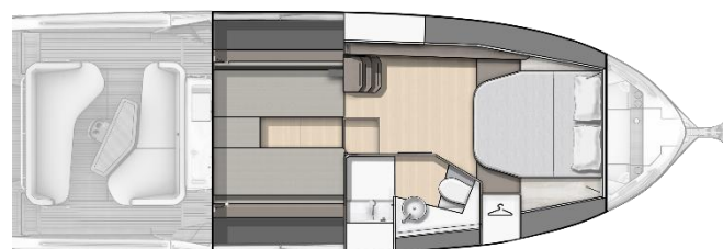
Lower deck
