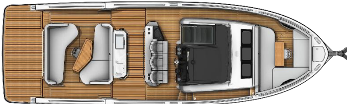
Main deck - Cockpit table version
